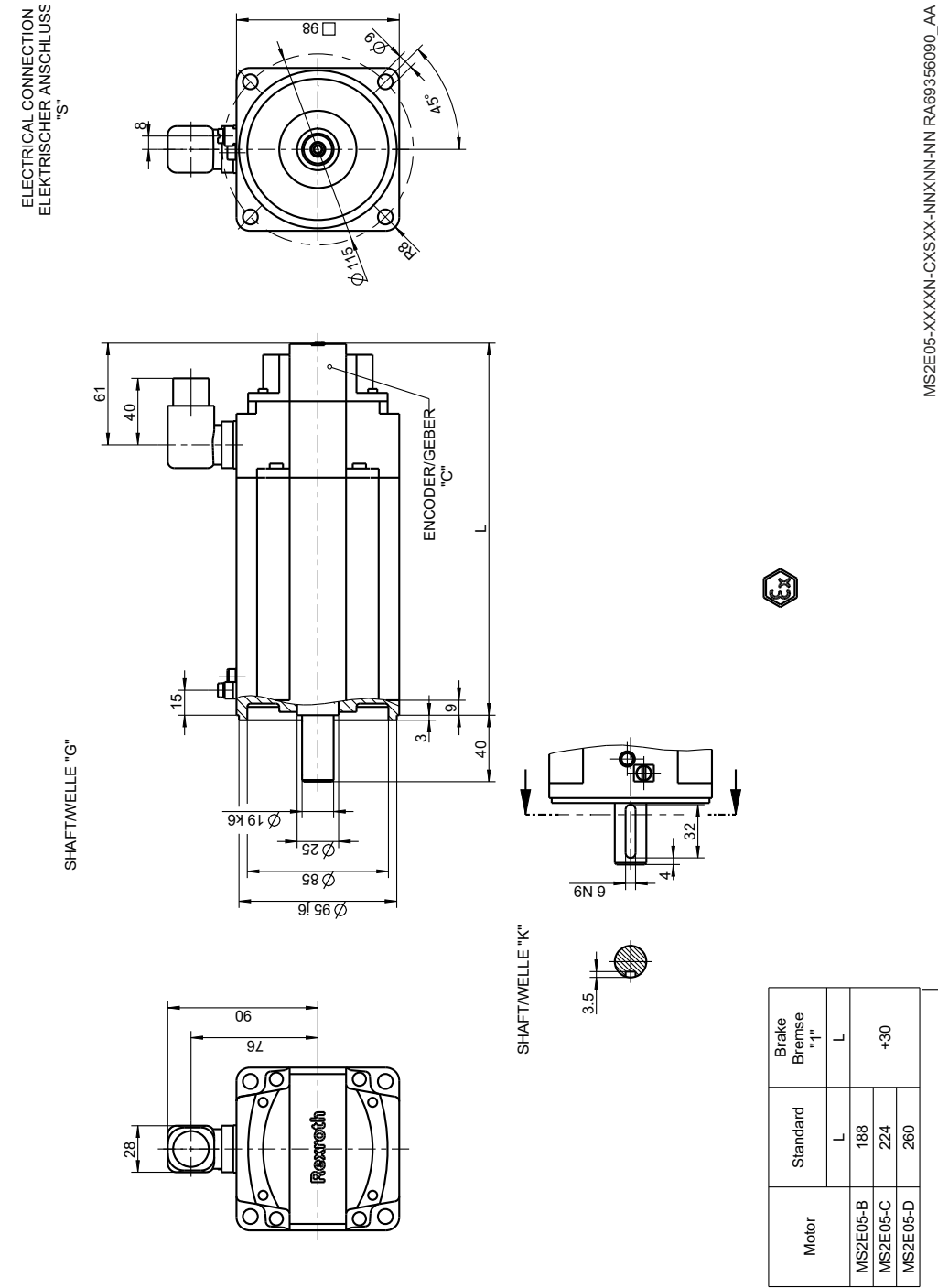
Fig. 44: MS2E05-xxxxN
