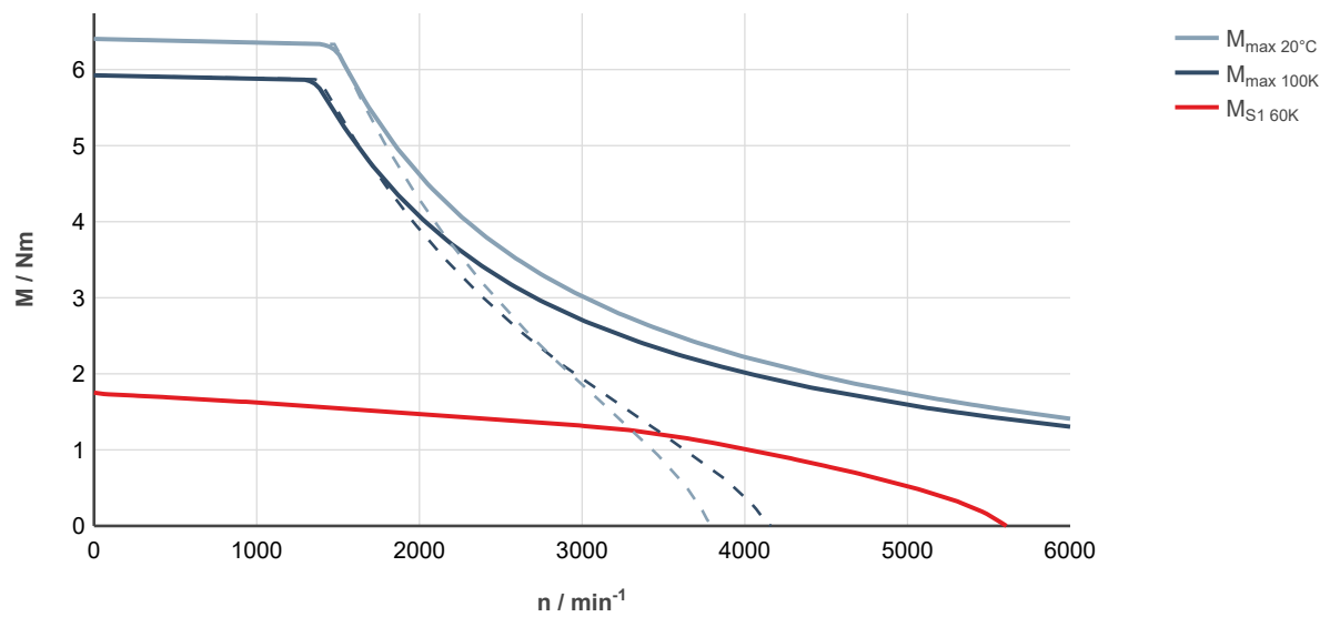
Fig. 27: MS2E04-B0BNN-___0-___-_, ctrlIX DRIVE, uncontrolled supply 3 x AC 400 V
