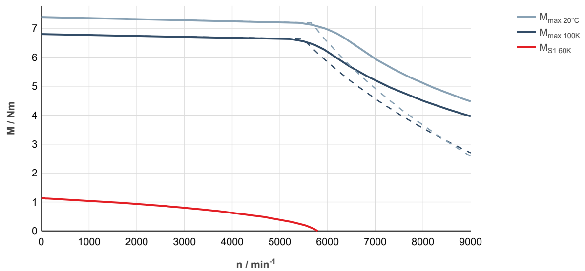
Fig. 22: MS2E03-D0BYN-___0-___-__, ctrlIX DRIVE, uncontrolled supply 3 × AC 400 V
