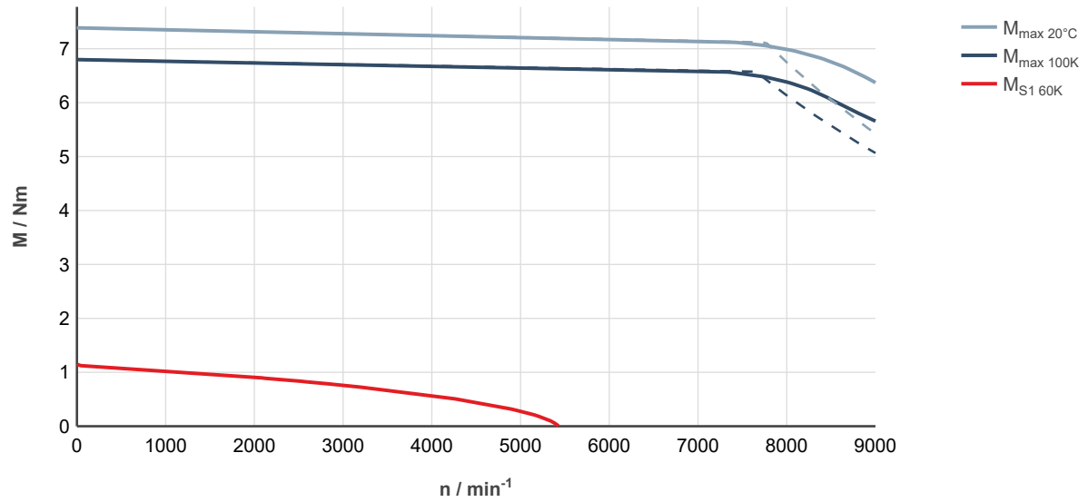
Fig. 23: MS2E03-D0BYN-___0-___-__, ctrlIX DRIVE, controlled supply 3 x AC 400 ... 480 V
