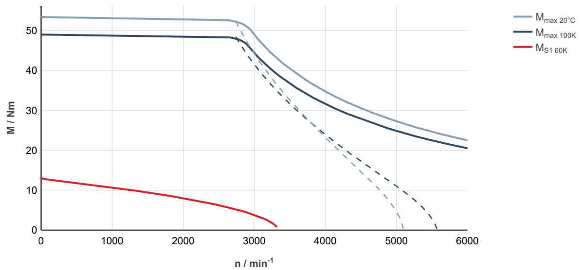
Fig. 54: MS2E06-E0BRN-___0-___-_, ctrlIX DRIVE, uncontrolled supply 3 x AC 400 V
