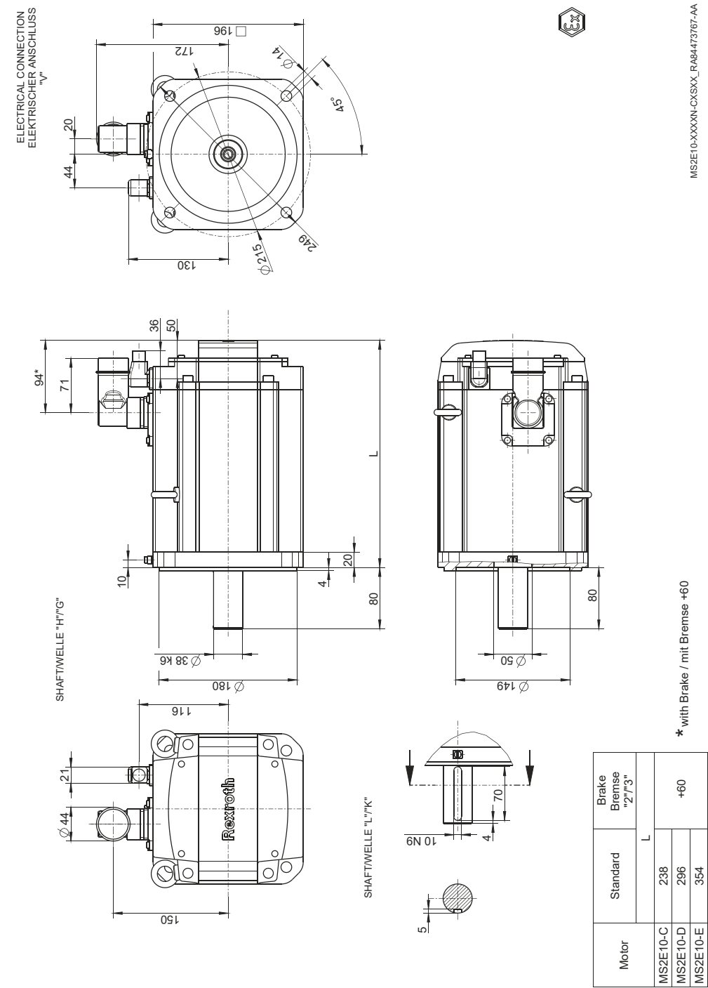
Fig. 86: MS2E10-XXXXN
