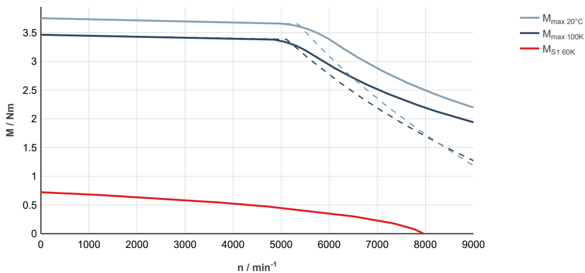
Fig. 20: MS2E03-B0BYN-___0-___-__, ctrlIX DRIVE, uncontrolled supply 3 × AC 400 V
