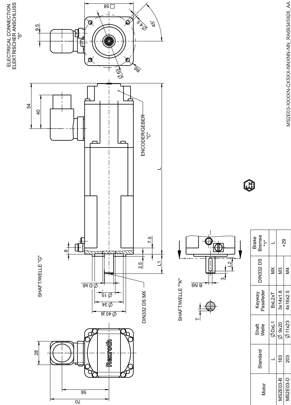
Fig. 24: MS2E03-xxxxN
