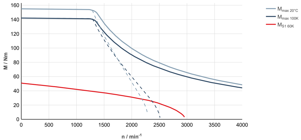
Fig. 78: MS2E10-D0BHN-___0-___-_, ctrlIX DRIVE, uncontrolled supply 3 × AC 400 V
