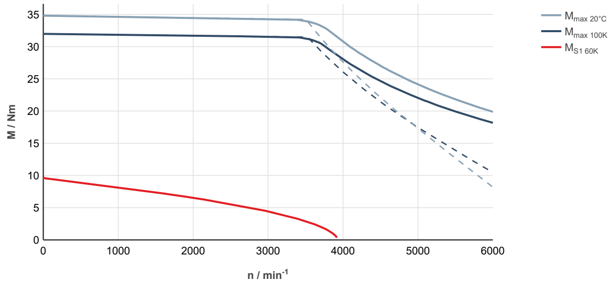
Fig. 53: MS2E06-D0BRN-___0-___-_, ctrlIX DRIVE, controlled supply 3 x AC 400 ... 480 V
