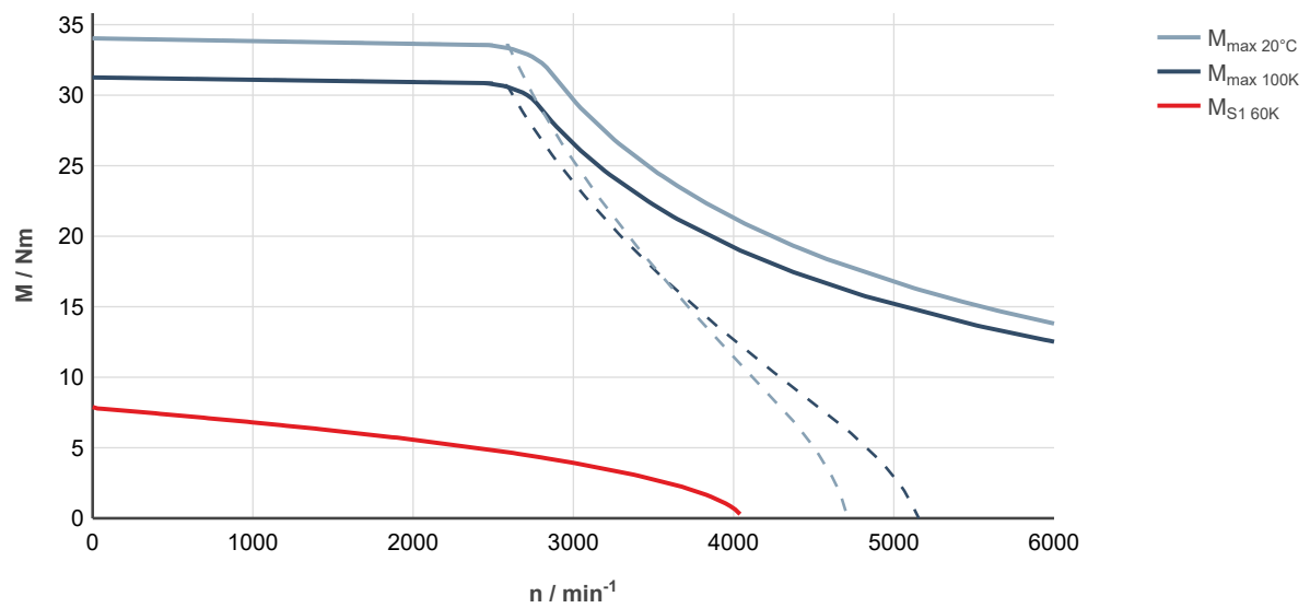
Fig. 42: MS2E05-D0BRN-___0-___-_, ctrlIX DRIVE, uncontrolled supply 3 × AC 400 V
