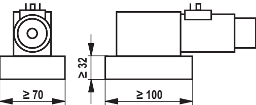
Individual assembly
