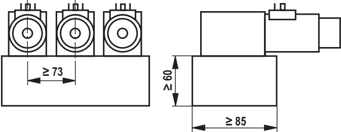
Bank assembly
