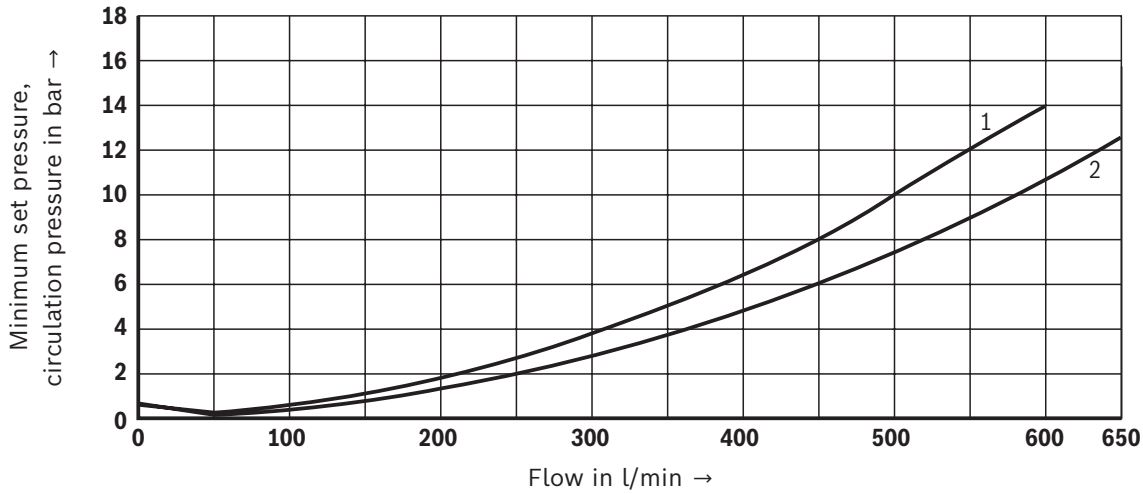
Minimum set pressure and circulation pressure dependent on the flow Version "U"
