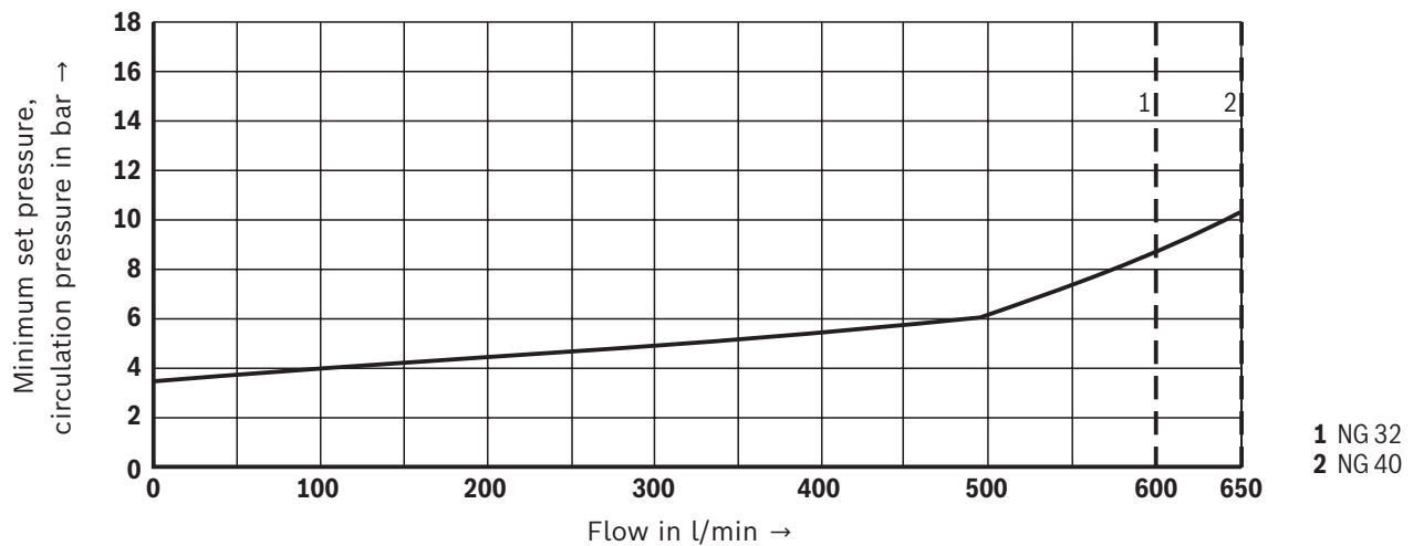
Minimum set pressure and circulation pressure dependent on the flow Standard version
