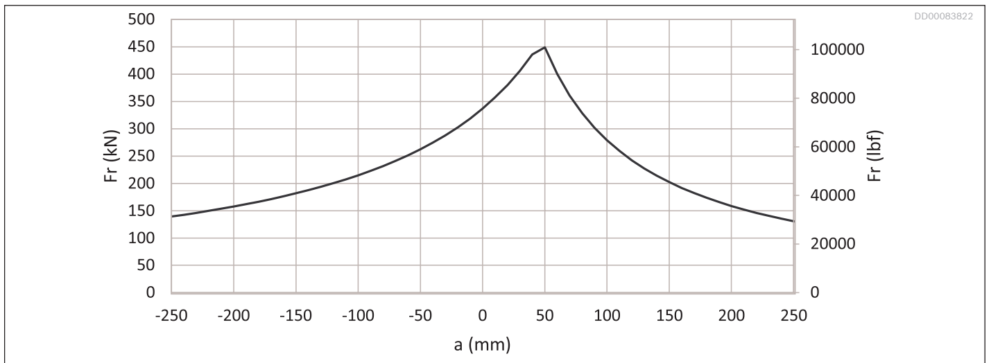
Fig. 39: Permissible external static load Häggglunds Atom 30 28 F and Atom 30 30 F (front flange)
