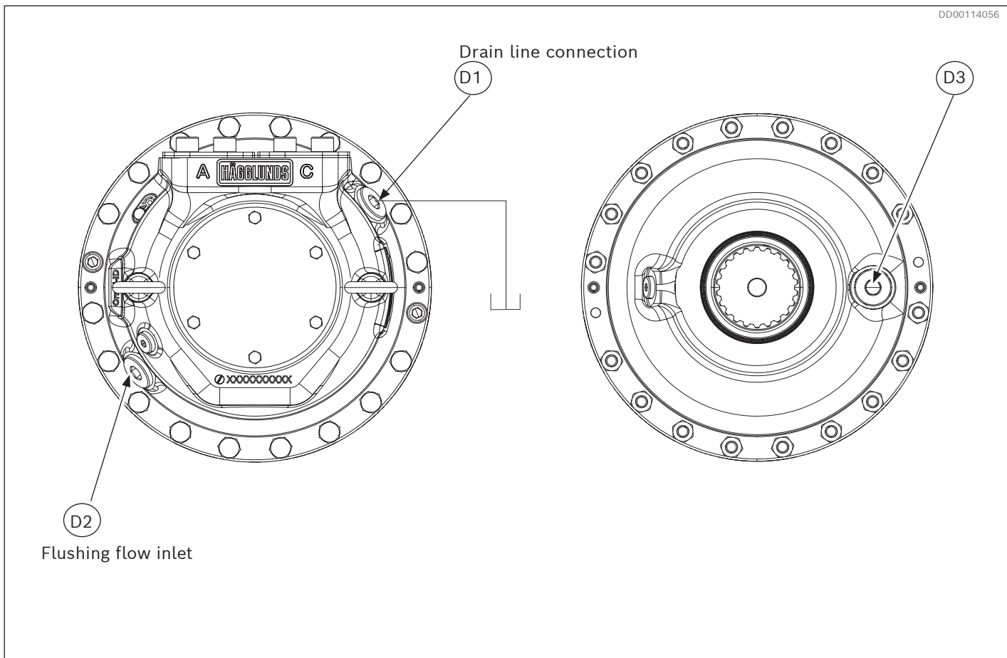
Fig. 23: Horizontal mounting
