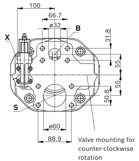
View Z
